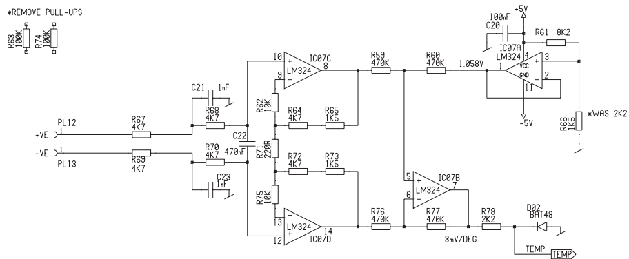
THERMOCOUPLE AMPLIFIER
